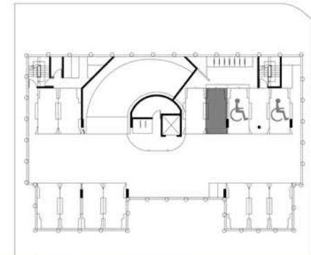
KEY PLAN - BASEMENT 2
